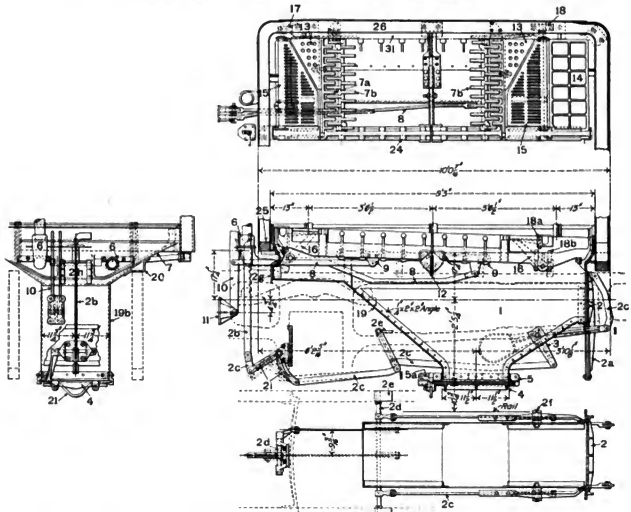
Figs. 546-549. General Arrangement of Ashpan and Shaking Grate. Atlantic (4-1-2) Locomotive. Pennsylvania Railroad.
